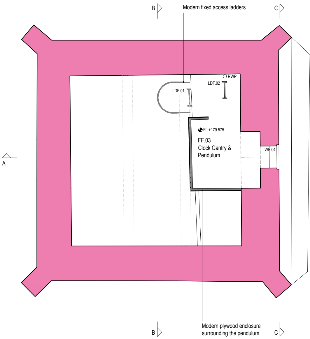
3 FIRST FLOOR CLOCK GANTRY PLAN AS EXISTING (10)/01 1:50
