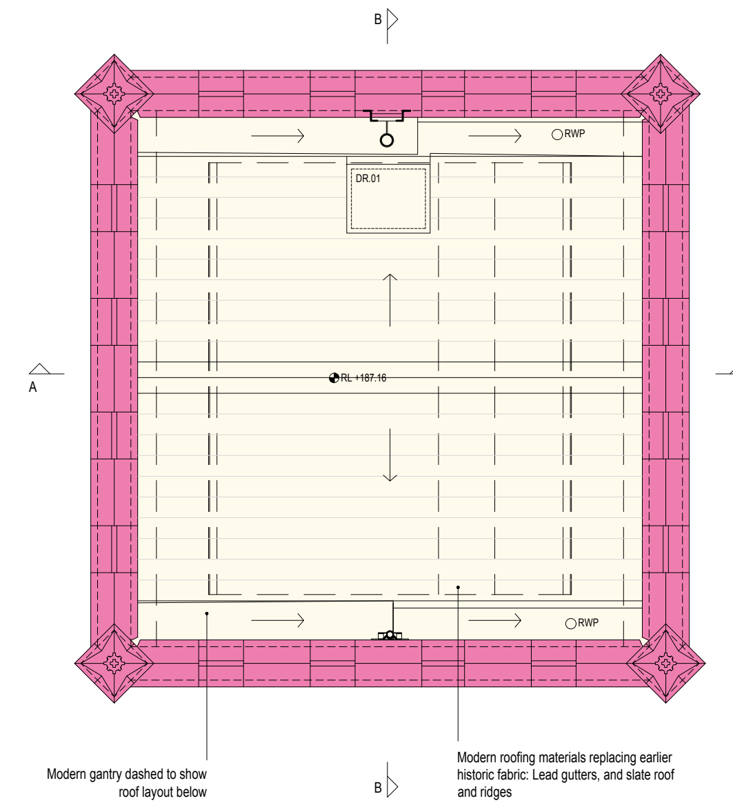
5 ROOF PLAN AS EXISTING (10)/01 1:50
