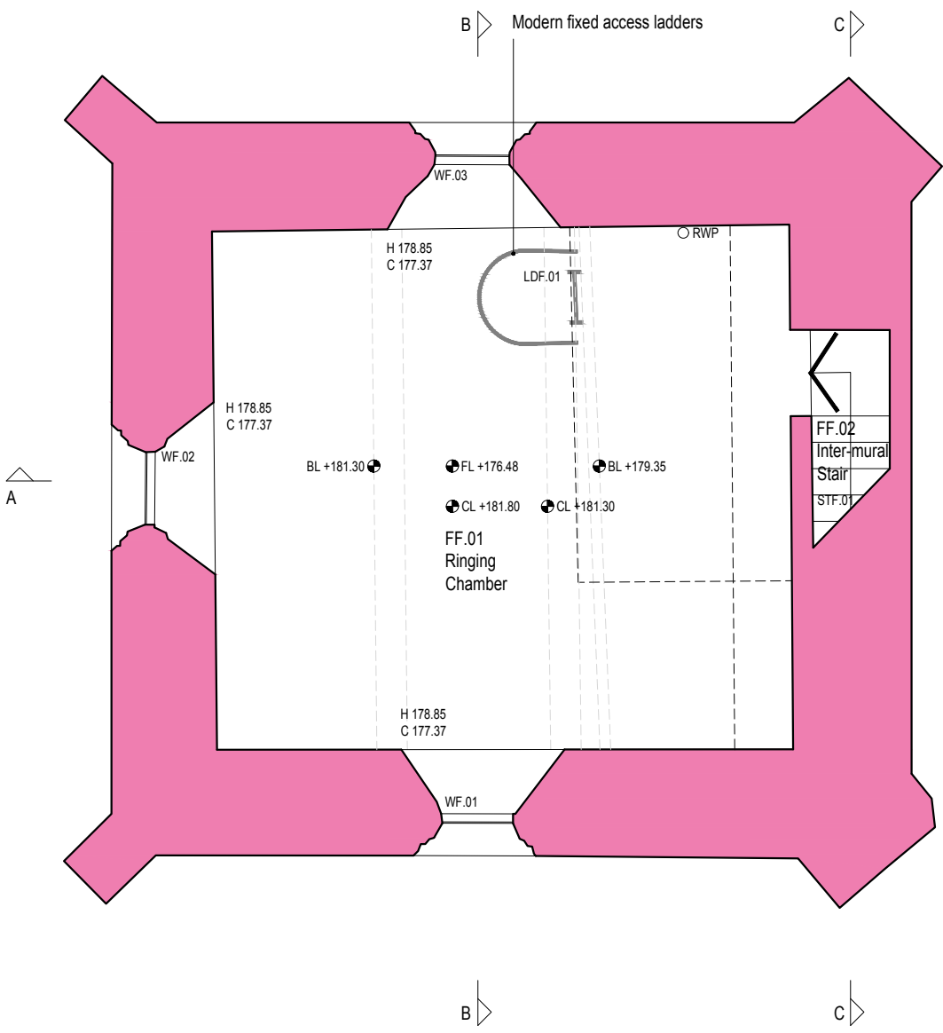
2 FIRST FLOOR PLAN AS EXISTING (10)/01 1:50
