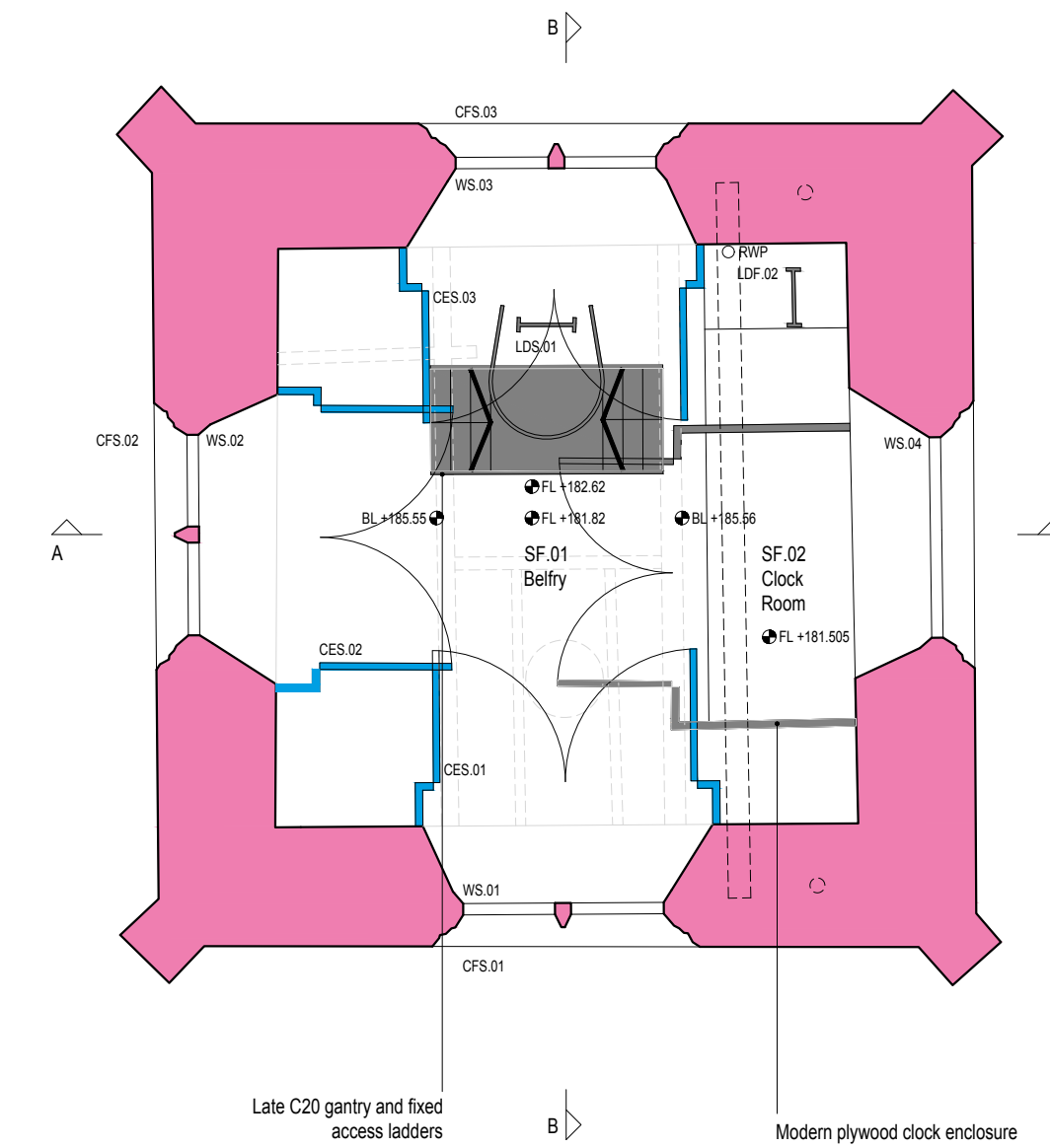
4 SECOND FLOOR PLAN AS EXISTING (10)/01 1:50
