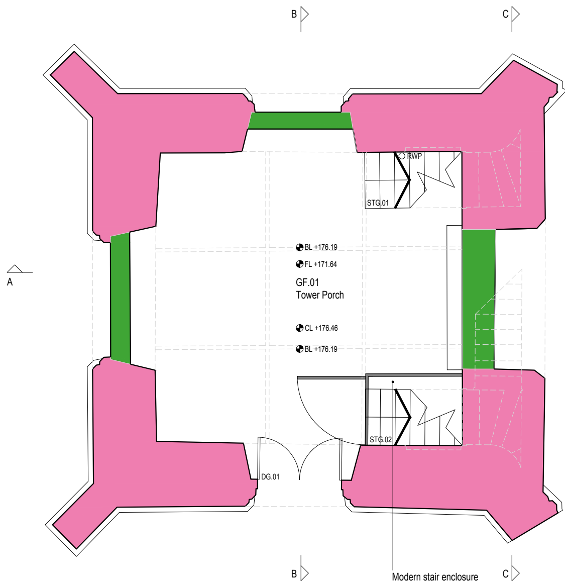
1 GROUND FLOOR PLAN AS EXISTING (10)/01 1:50
